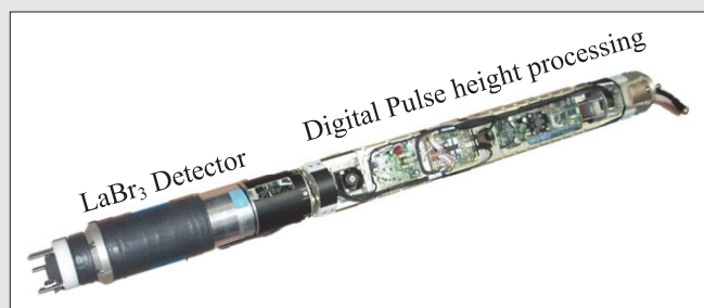
Figure 8. Detector Module – view \text{LaBr}_3 and digital processing electronic board
